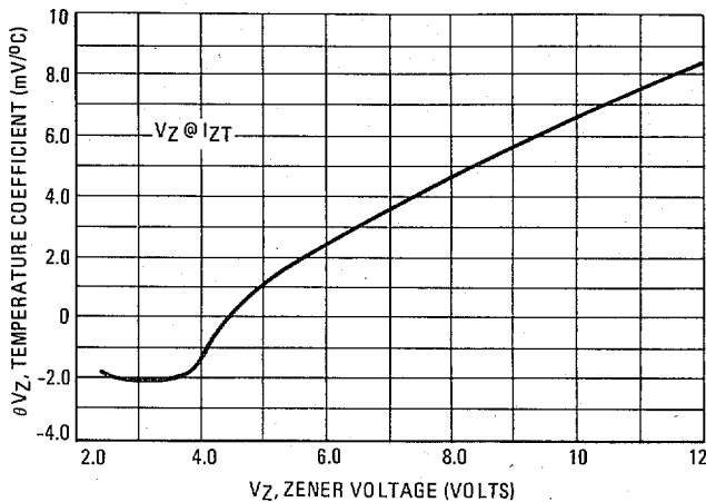
FIGURE 2A – ZENER VOLTAGE 2.4 to 12 VOLTS
