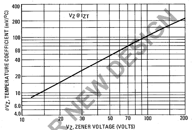
FIGURE 2B – ZENER VOLTAGE 12 to 200 VOLTS
