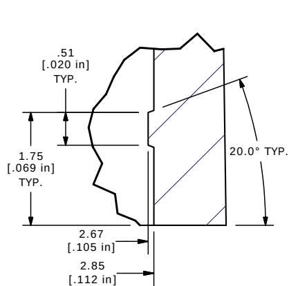
DETAIL C SCALE 16 : 1
