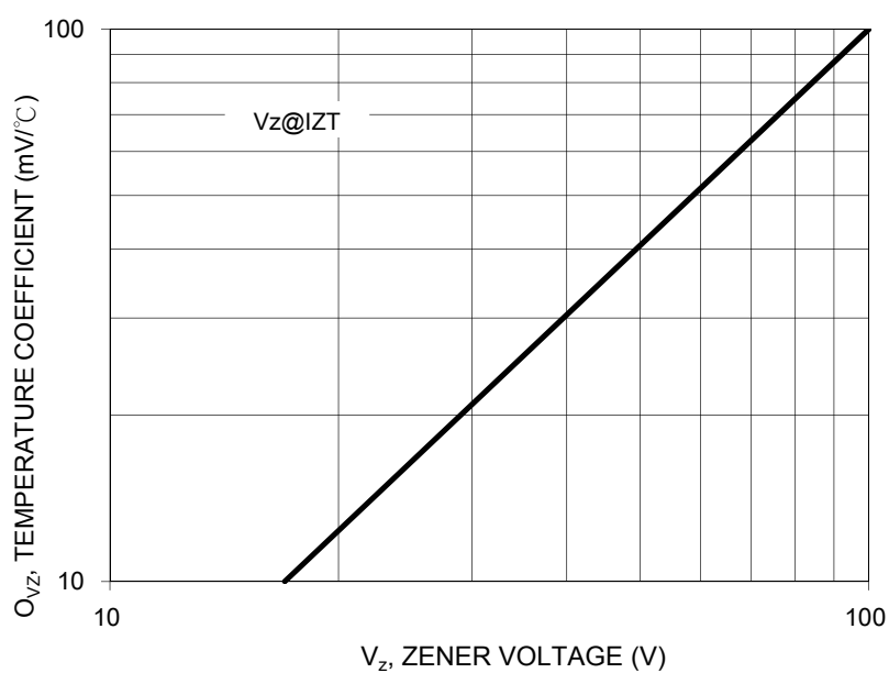
FIG.4 ZENER VOLTAGE 14 TO 200 VOLTAGES
