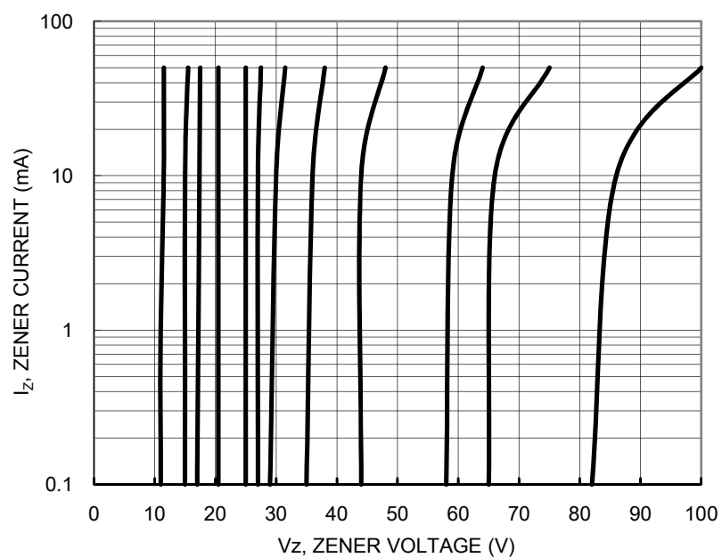
FIG. 6 V_Z = 12 THRU 82 VOLTS
