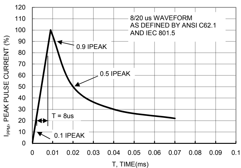
FIG. 12 PULSE WAVEFORM
