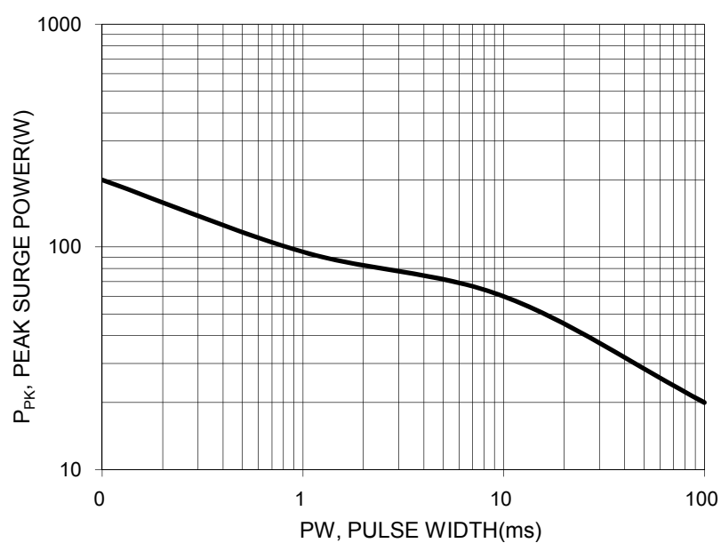
FIG.2 MAXIMUM SURGE POWER
