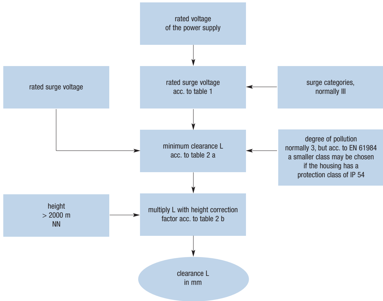
Diagram for the Determination of Clearances
