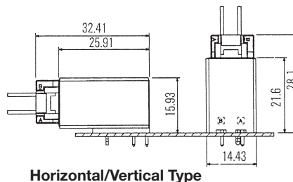
Horizontal/Vertical Type
