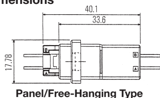
Panel/Free-Hanging Type
