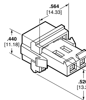
Two-Position Only 641533-1
