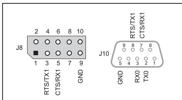
Figure 3-17. RS-232 Signals
