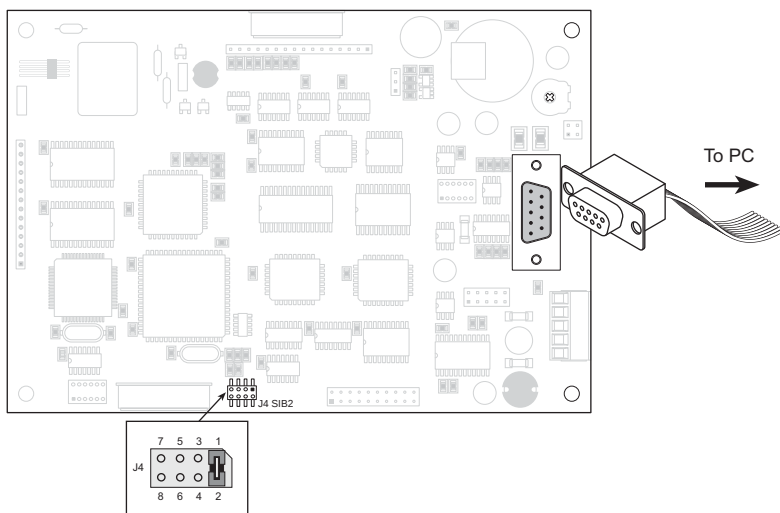
Figure 2-5. Direct Programming Connection
