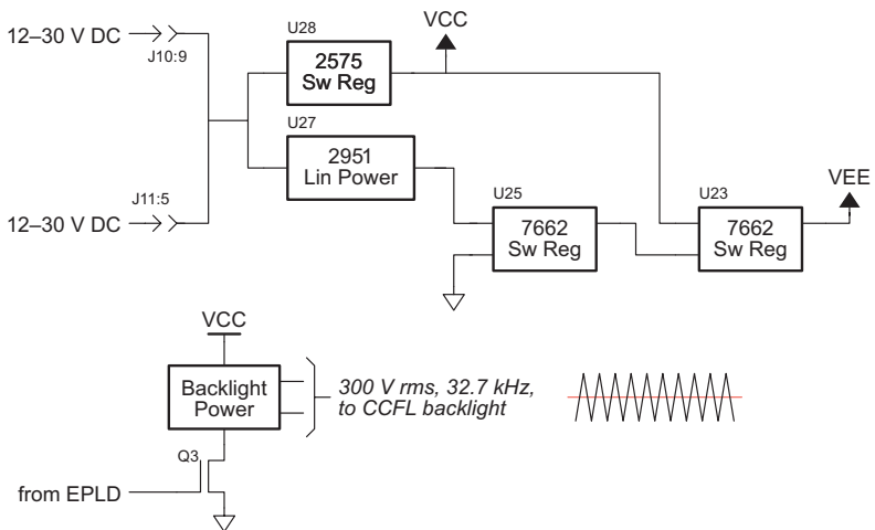
Figure 3-2. Block Diagram of OP7100 Internal Power Regulators
