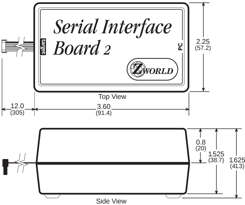
Figure D-1. SIB External Dimensions
