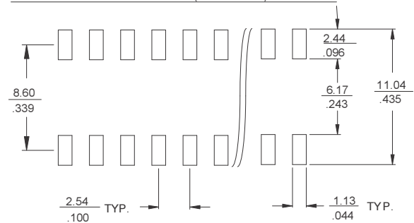
SURFACE MOUNT PAD LAYOUTS (ALL STYLES)
