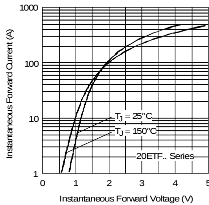
Fig. 7 - Forward Voltage Drop Characteristics
