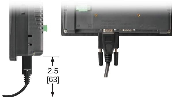
Standard Cable With Right Angle Adapter
