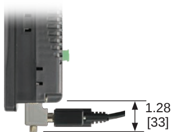
Standard Cable With Right Angle Adapter
