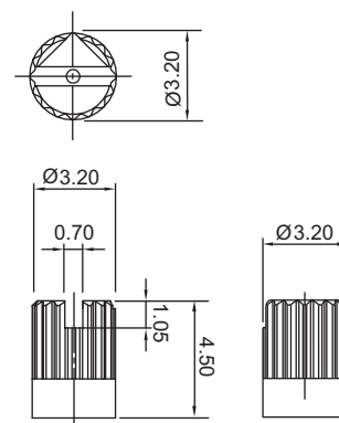
C: KNURLED, SLOTTED SHAFT
