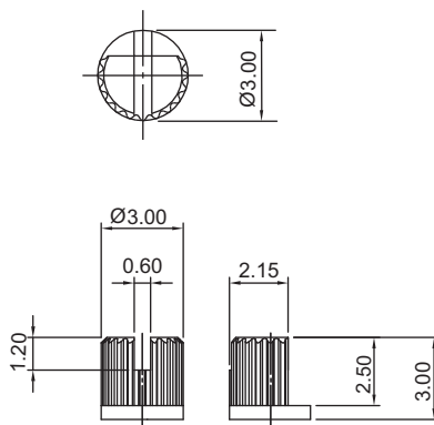
B: KNURLED, SLOTTED, FLATTED SHAFT
