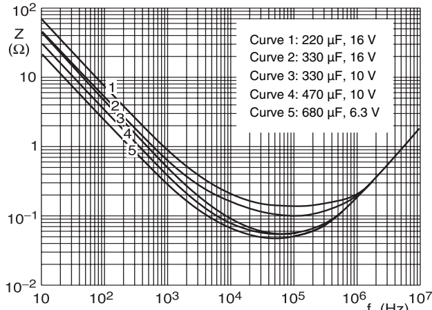
Case \varnothing D \times L = 10.3 \times 32.0 mm; U_R = 6.3 to 16 V T_{\text{amb}} = 25 °C Fig.15 Typical impedance as a function of frequency
