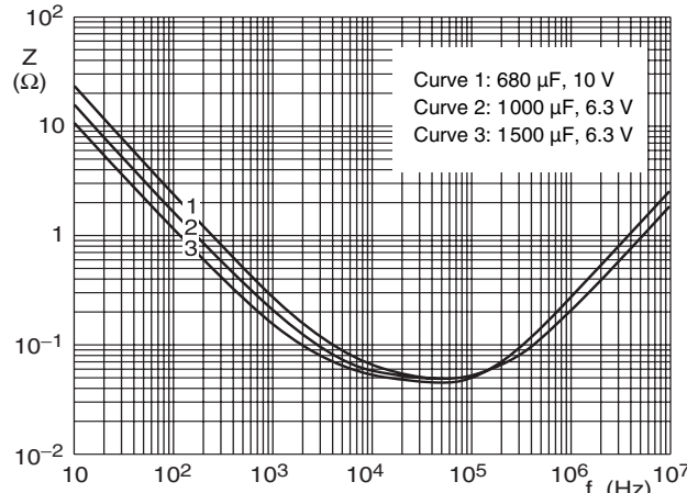
Case \varnothing D \times L = 12.9 \times 32.0 mm; U_R = 6.3 to 10 V T_{\text{amb}} = 25 °C Fig.17 Typical impedance as a function of frequency
