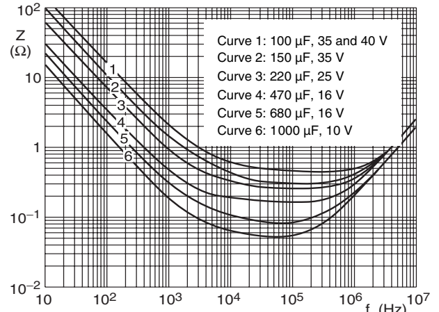
Case \varnothing D \times L = 12.9 \times 32.0 mm; U_R = 10 to 40 V T_{\text{amb}} = 25 °C Fig.18 Typical impedance as a function of frequency
