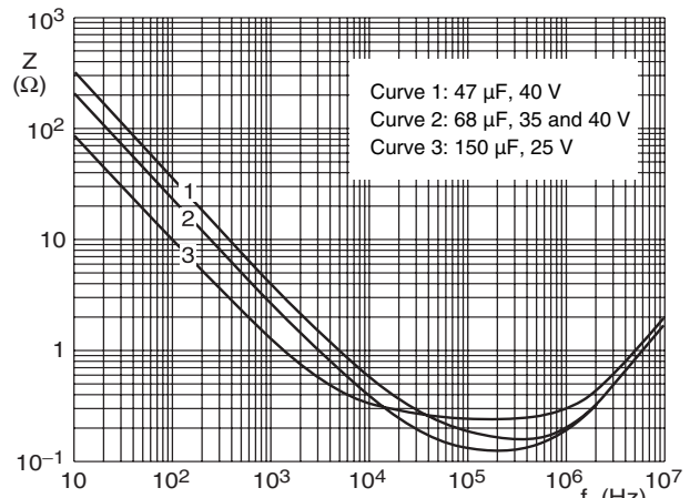
Case \varnothing D \times L = 10.3 \times 32.0 mm; U_R = 25 to 40 V T_{\text{amb}} = 25 °C Fig.16 Typical impedance as a function of frequency
