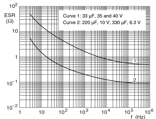
Case \varnothing D \times L = 9.4 \times 23.3 mm T_{amb} = 25 °C Fig.26 Typical ESR as a function of frequency
