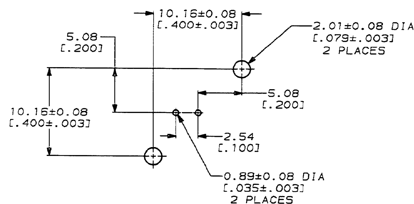
PCB CONFIGURATION
