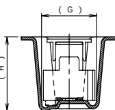
SECT. F-F
