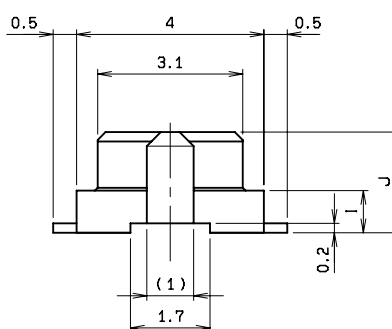
SECT. E-E
