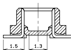
SECT. E-E
