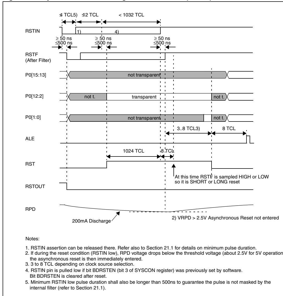
Figure 22. Synchronous short / long hardware RESET ( \overline{\text{EA}} = 0 )
