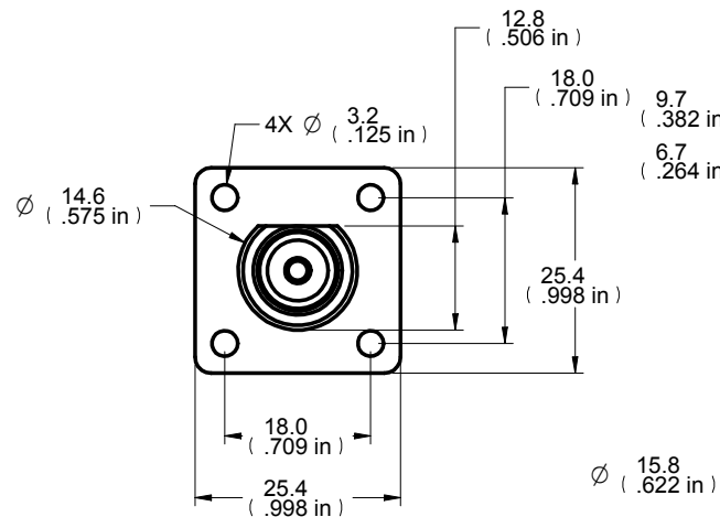
DIM OUTLINE
