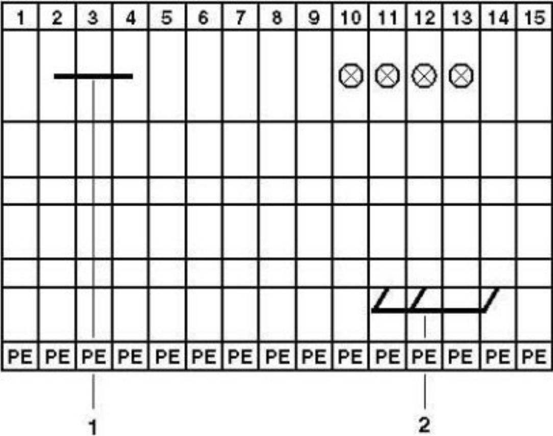
Circuit diagram
