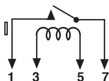
Figure A SPST-NO Without diode
