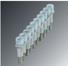
Fixed bridge, pitch: 6 mm, number of positions: 10, color: silver
