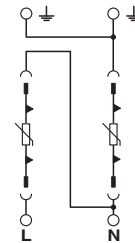
Circuit diagram
