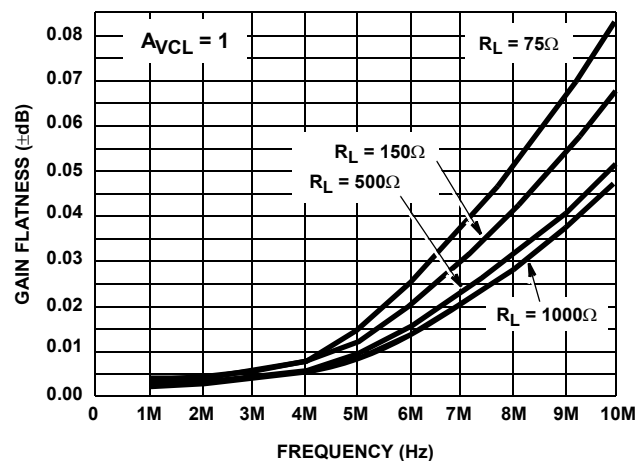
FIGURE 20. GAIN FLATNESS vs FREQUENCY
