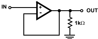
TEST CIRCUIT
