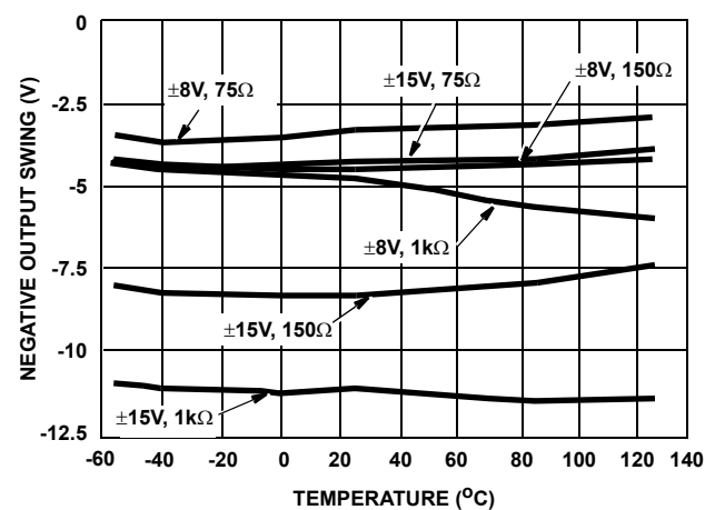
FIGURE 14. NEGATIVE OUTPUT SWING vs TEMPERATURE
