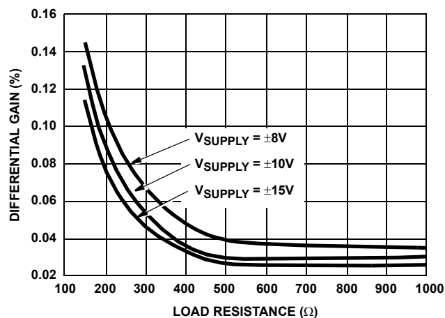
FIGURE 18. DIFFERENTIAL GAIN vs LOAD RESISTANCE
