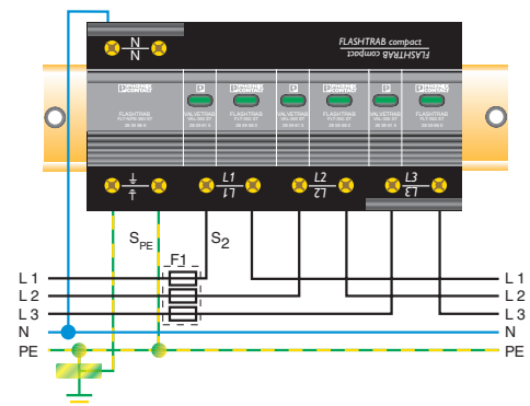
V wiring connection
