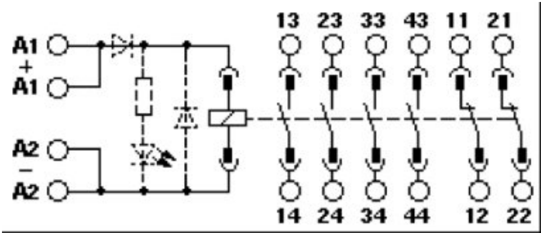
Circuit diagram
