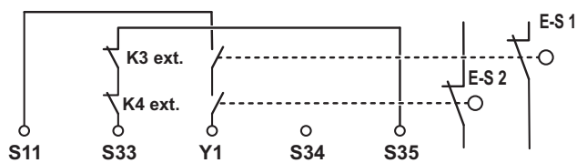
Figure 20 Automatic activation with restart inhibit in the event of mains failure (E-S1, E-S2) with monitored contact extension (K3 ext., K4 ext.) Not fault-proof
