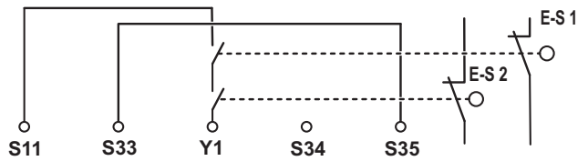
Figure 18 Automatic activation with restart inhibit in the event of mains failure (E-S1, E-S2) Not fault-proof
