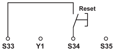
Figure 13 Monitored reset
