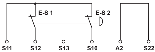
Figure 23 Two-channel without cross-circuit detection, two N/C contacts
