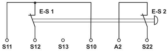
Figure 21 Two-channel with cross-circuit detection, two N/C contacts
