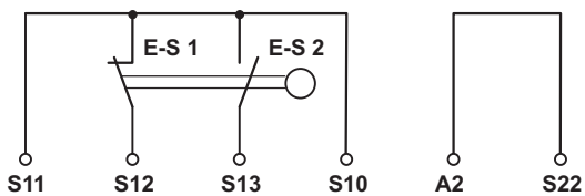
Figure 25 Two-channel without cross-circuit detection, one N/C contact and one N/O contact
