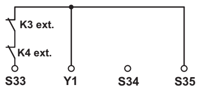
Figure 16 Automatic activation with monitored contact extension (K3 ext., K4 ext.)
