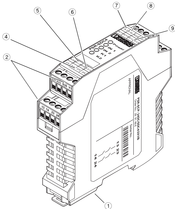
PSR-SCP- 24DC/SDC4/2X1/B
