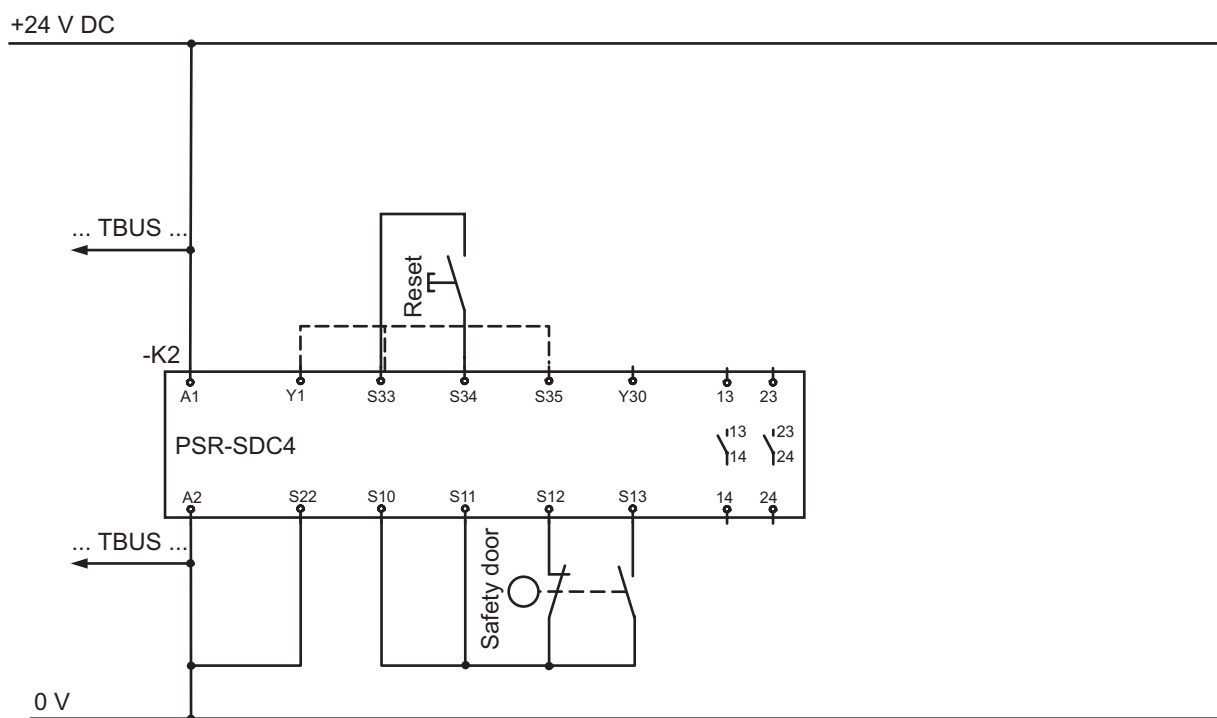
Figure 8 Two-channel safety door monitoring without cross-circuit detection, one N/C contact and one N/O contact
