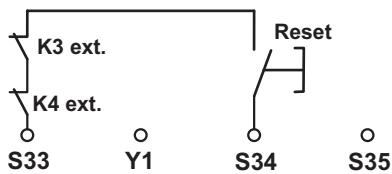
Figure 17 Monitored reset with monitored contact extension (K3 ext., K4 ext.)
