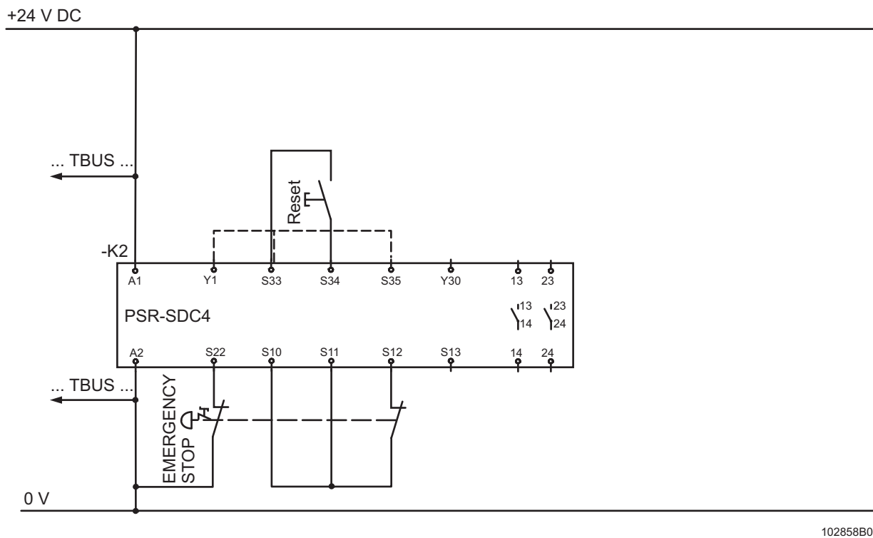
Figure 6 Two-channel emergency stop circuit (2 N/C contacts) with cross-circuit detection
