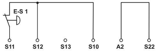
Figure 22 Single-channel
