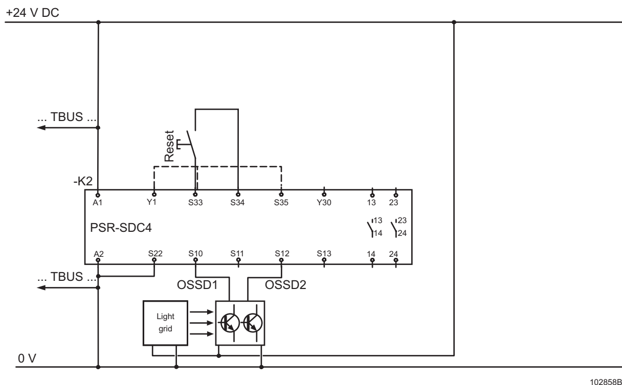
Figure 12 Two-channel light grid monitoring with cross-circuit detection
