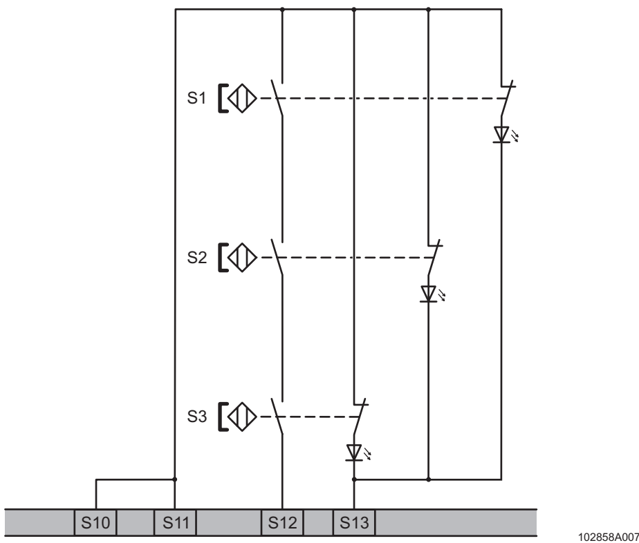
Figure 10 Connection for safety category 3 according to EN 954-1: Example with three magnetic switches with 2-pos. control switch (N/C contact and N/O contact), with open safety door
