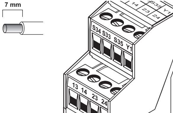
Figure 4 PSR-SCP- 24DC/SDC4/2X1/B
