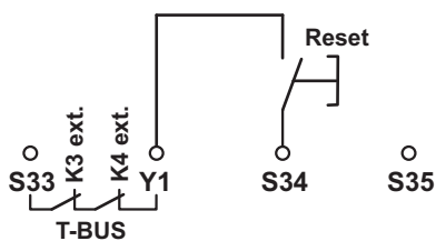
Figure 15 Monitored reset with monitored contact extension (K3 ext., K4 ext.) via T-BUS DIN rail connector
