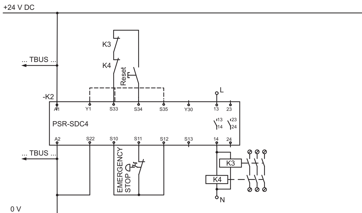
Figure 11 Single-channel emergency stop circuit with monitored contact extension
