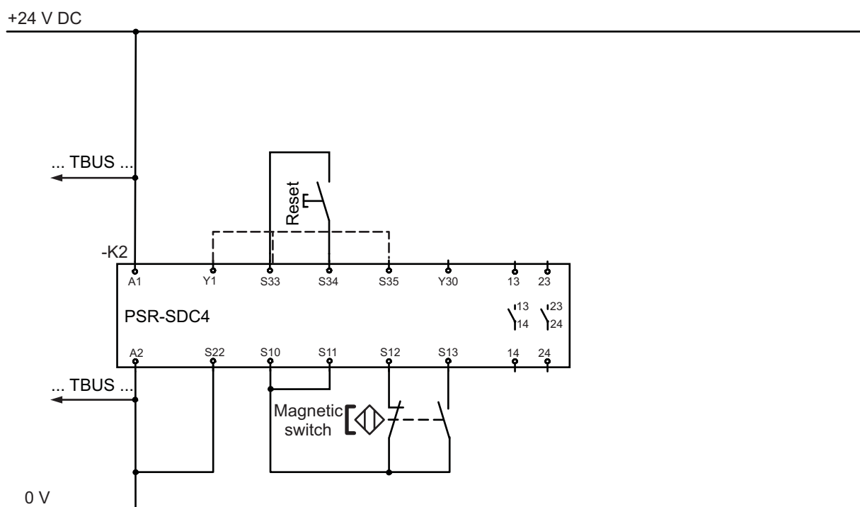
Figure 9 Monitoring with encoded magnetic switch without cross-circuit detection, with closed safety door
