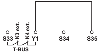
Figure 14 Automatic activation with monitored contact extension (K3 ext., K4 ext.) via T-BUS DIN rail connector
