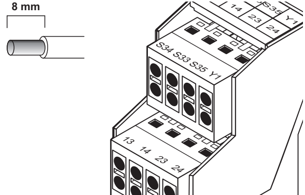
Figure 5 PSR-SPP- 24DC/SDC4/2X1/B
