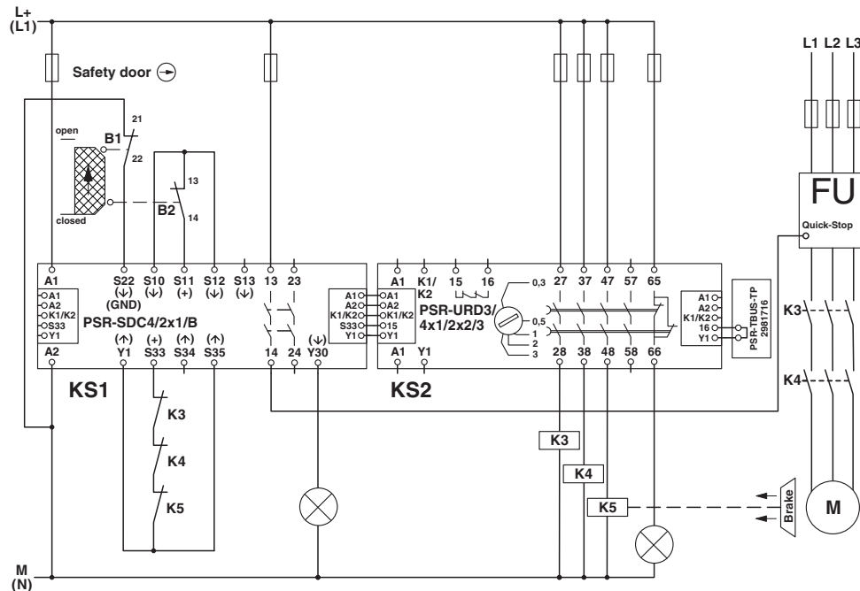
Circuit diagram
