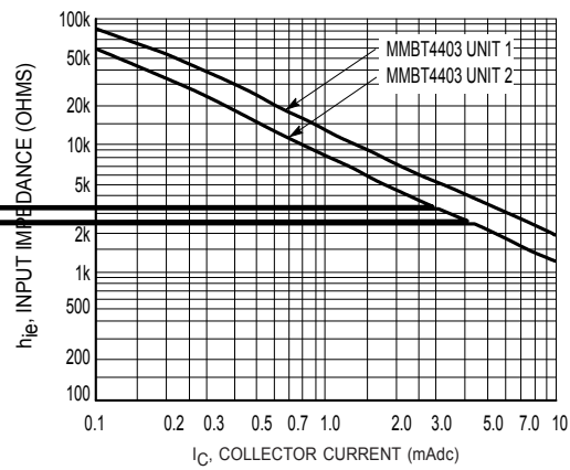
Figure 9. Input Impedance
