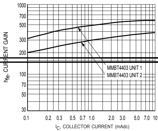
Figure 8. Current Gain
