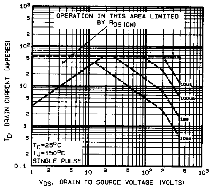
Fig 8. Maximum Safe Operating Area
