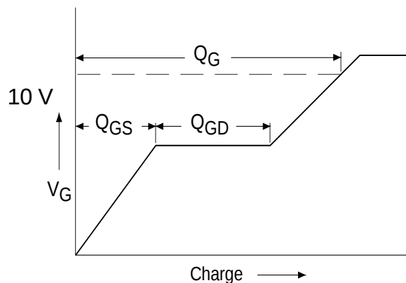
Fig 13a. Basic Gate Charge Waveform
