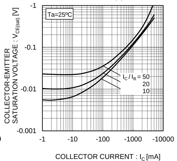
Fig.6 Collector-Emitter Saturation Voltage vs. Collector Current (II)
