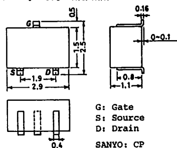
Case Outline—[2050] unit: mm
