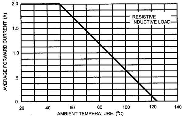
FIG.2- MAXIMUM CURRENT DERATING CURVE OUTPUT RECTIFIED CURRENT
