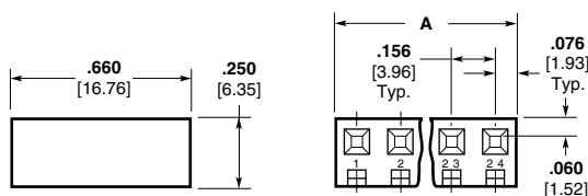
(C) Without Locking Ramp/Without Polarizing Tabs
