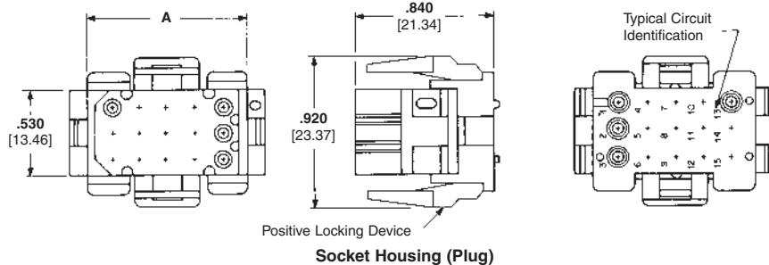
Socket Housing (Plug)
