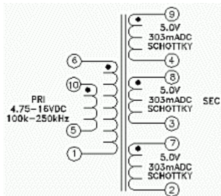
Schematic 1
