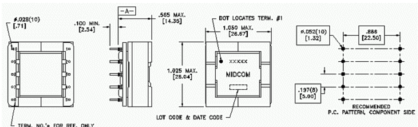
Mechanical 3
