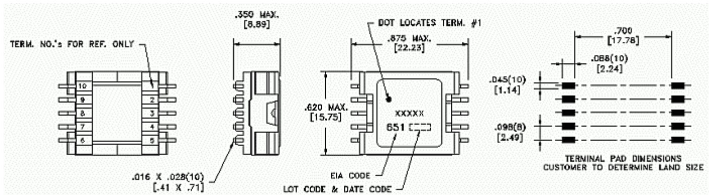
Mechanical 1
