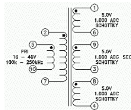
Schematic 2
