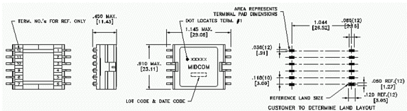
Mechanical 2
