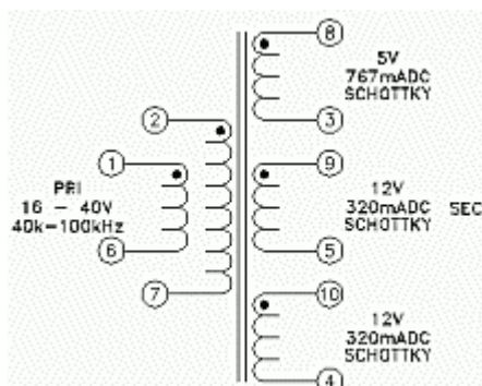
Schematic 5
