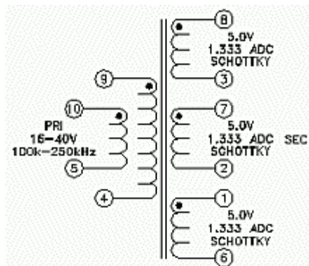
Schematic 3
