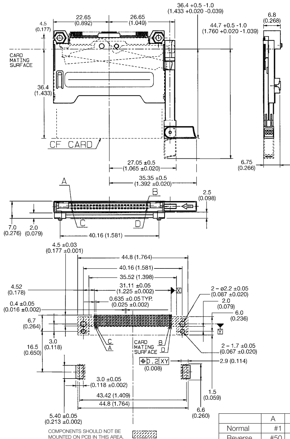
RECOMMENDED PRINTED CIRCUIT LAYOUT
