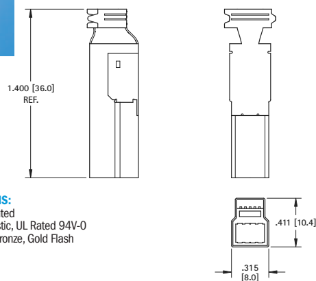
CABLE PLUG
