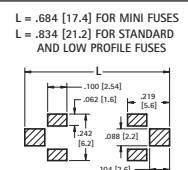
Mounting Detail For Two Clips
