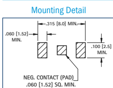
4.8mm CELL
