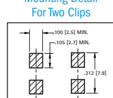
Mounting Detail For Two Clips
