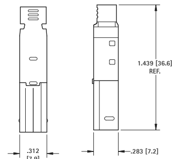
CABLE PLUG
