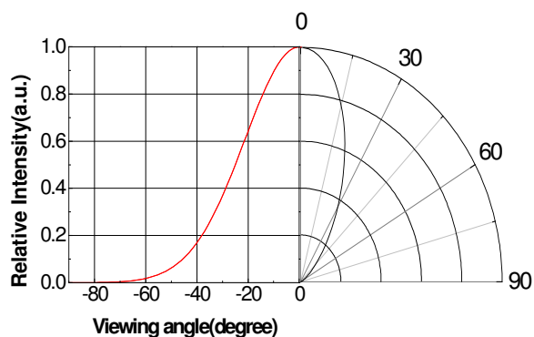
Radiation Characteristics
