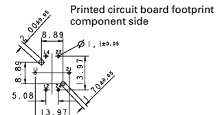
view on component side PCB
