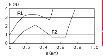
FORCE/TRAVEL DIAGRAM
