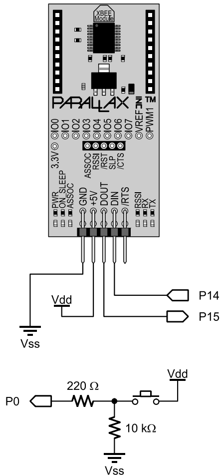
Transmitter Configuration
