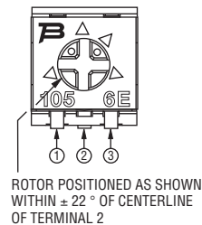
3314S-4 (Reverse Marking, Cross Slot)
