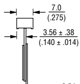
SIDE VIEW 3362U-1
