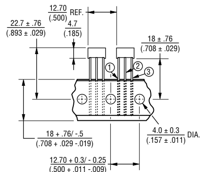
SIDE VIEW 3362U-1
