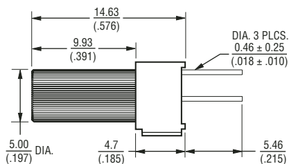
TOP ADJUST 3362U-1, 3362P-1
