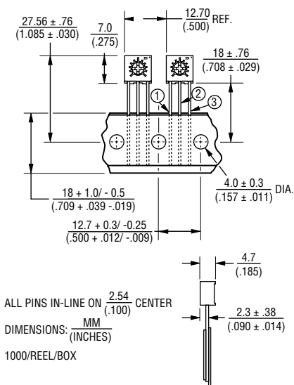
TOP ADJUST 3362U-1, 3362P-1
