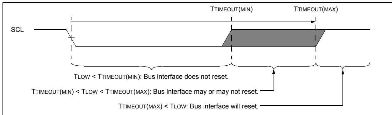
FIGURE 4-2: BUS TIMEOUT
