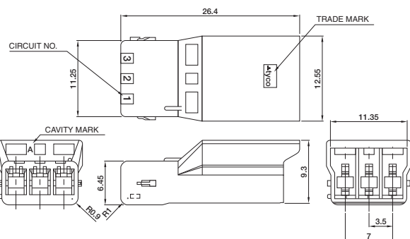
Cap Housing (For Tabs)
