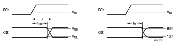
SCK to SDO Delay
