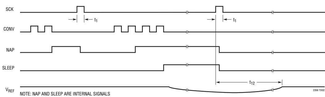
Nap Mode and Sleep Mode Waveforms
