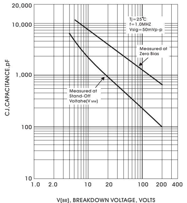
FIGURE 4 TYPICAL CAPACITANCE VS STAND-OFF VOLTAGE
