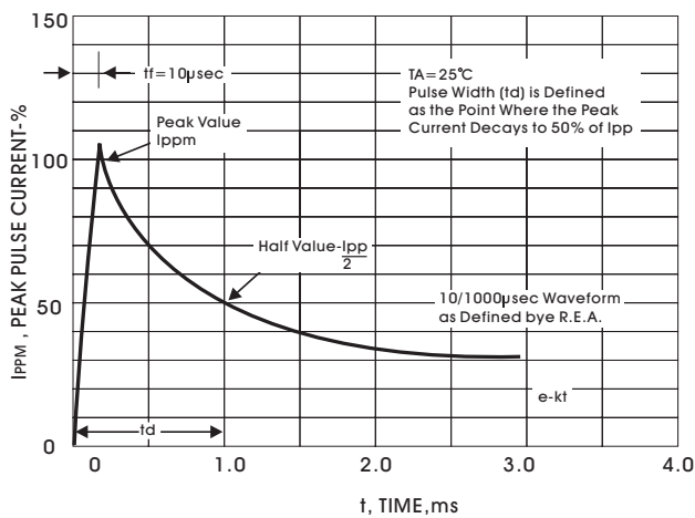
FIGURE 3-PULSE WAVEFORM
