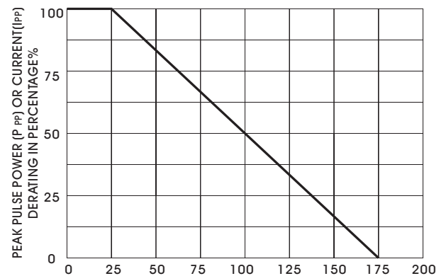
FIGURE 2 DERATING CURVE
