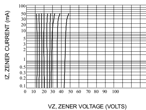
Fig. 7-VZ = 12 THRU 40 VOLTS
