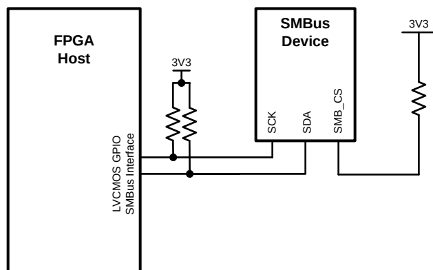
Figure 8. SMBus Configuration 1
