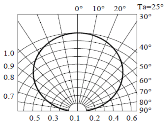
Radiation Diagram
